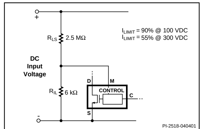
Figure 18. Current Limit Reduction with Line Voltage.
