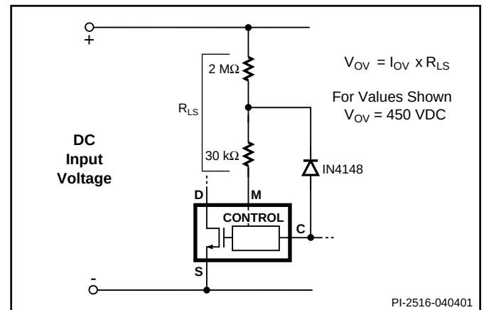
Figure 16. Line Sensing for Overvoltage Only (Under-Voltage Disabled).
