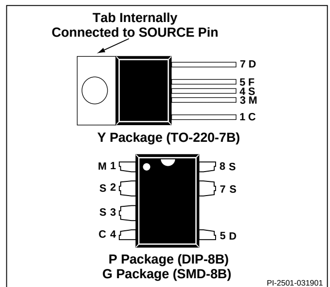
Figure 3. Pin Configuration.
