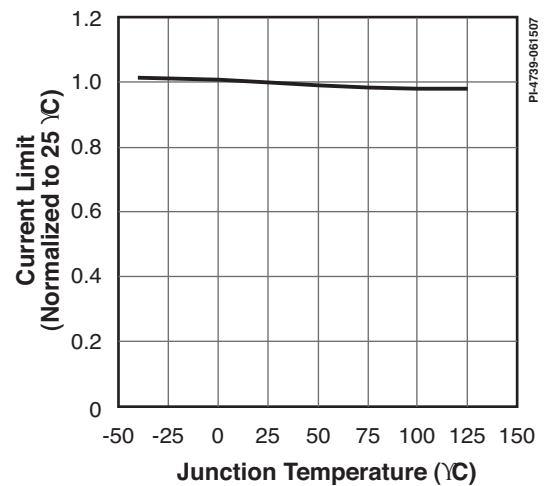
Figure 59. External Current Limit vs. Temperature with R_{IL} = 10.5 \text{ k}\Omega .
