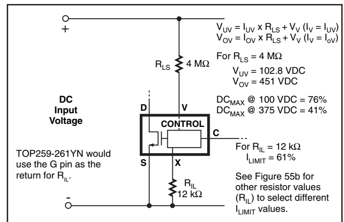
Figure 27. Line Sensing and Externally Set Current Limit.
