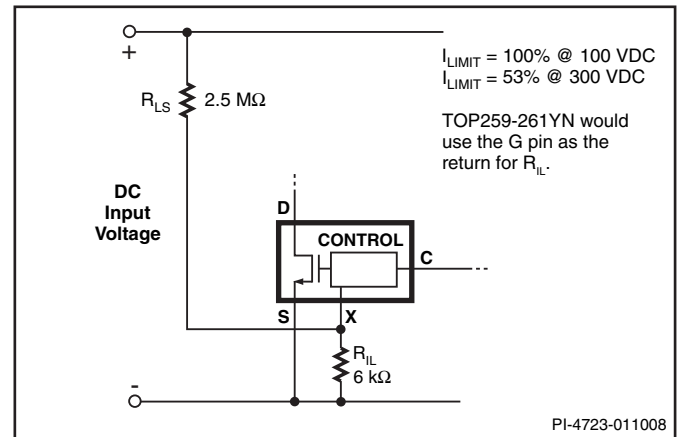
Figure 23. Current Limit Reduction with Line Voltage.
