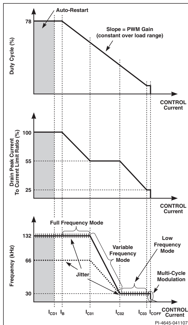
Figure 9. Control Pin Characteristics (Multi-Mode Operation).
