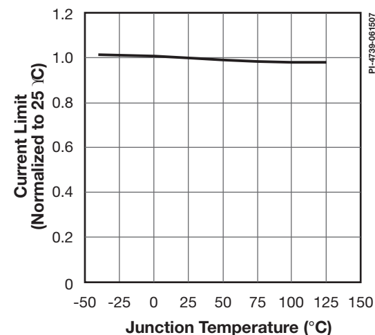
Figure 41. External Current Limit vs. Temperature with R_{IL} = 10.5 \text{ k}\Omega .
