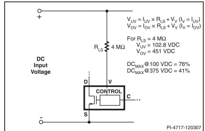
Figure 14. Line-Sensing for Undervoltage, Overvoltage and Line Feed-Forward.
