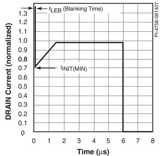
Figure 34. Drain Current Operating Envelope.
