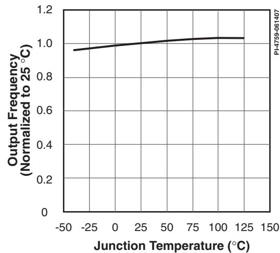
Figure 39. Frequency vs. Temperature.
