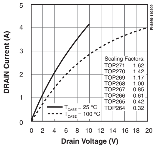
Figure 48. Output Characteristics.
