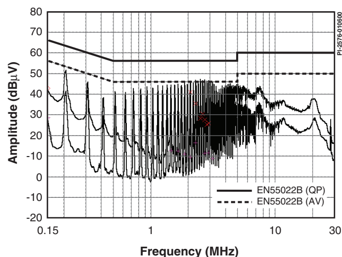
Figure 27. Fixed Frequency Operation Without Jitter.
