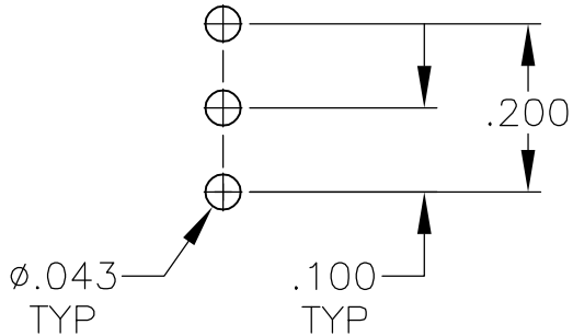
RECOMMENDED PCB LAYOUT TOLERANCES \pm .002
