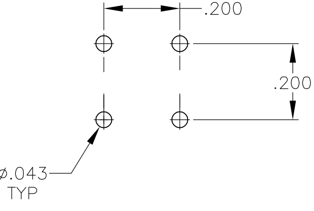
RECOMMENDED PCB LAYOUT TOLERANCES +/- .002
