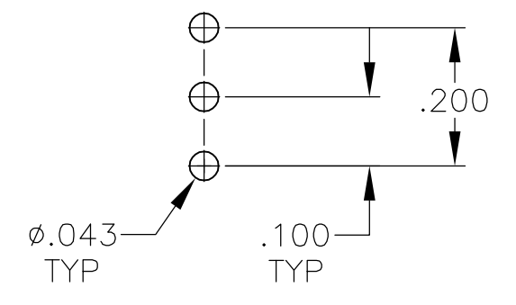
RECOMMENDED PCB LAYOUT TOLERANCES +/- .002
