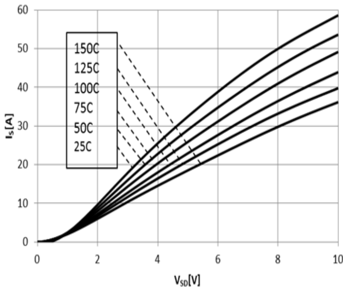
Figure 7. Forward Characteristics of Rev. Diode
