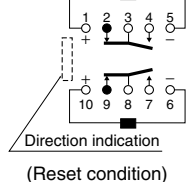
2-coil latching
