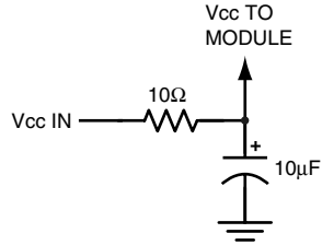
Figure 15: Supply Filter
