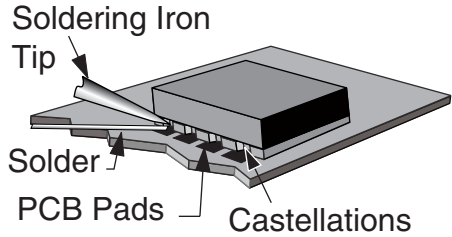
Figure 21: Soldering Technique
