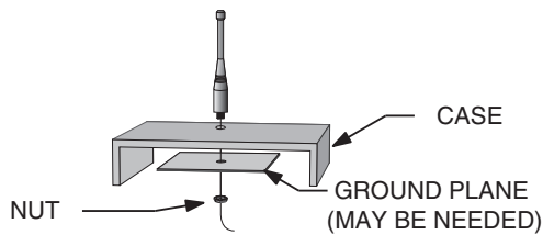
Figure 26: Remote Ground Plane
