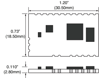
Figure 1: Package Dimensions
