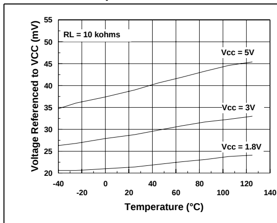
Figure 19. High level output voltage vs. temperature
