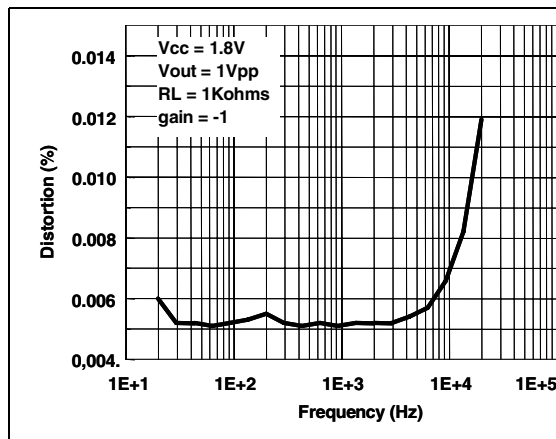
Figure 43. Distortion vs. frequency at V_{CC} = 1.8\text{ V}
