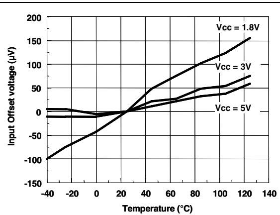
Figure 2. Input offset voltage vs. temperature
