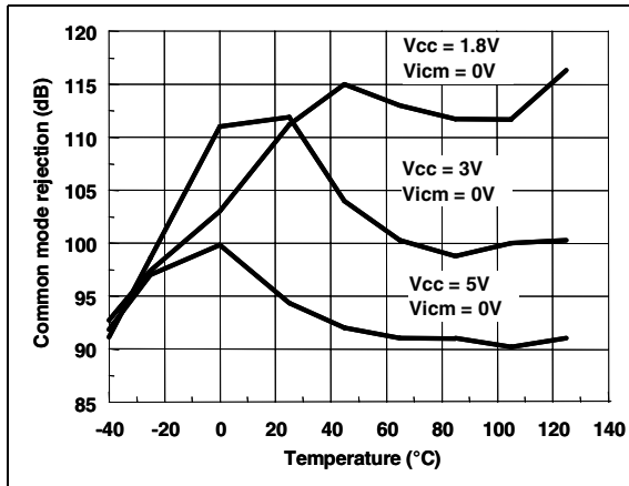
Figure 7. Common mode rejection vs. temperature
