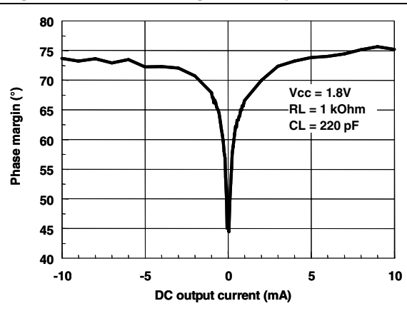
Figure 34. Phase margin vs. output current
