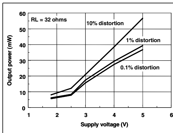
Figure 47. Output power vs. supply voltage
