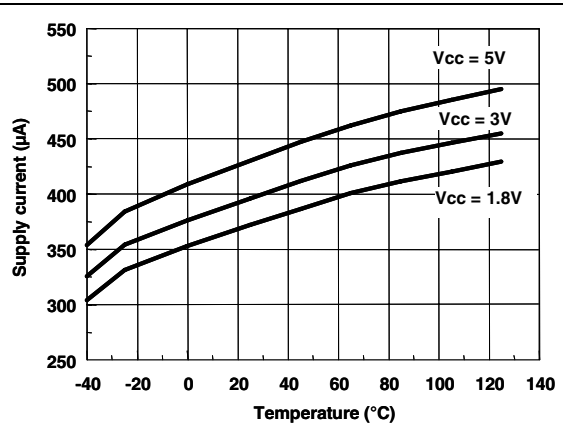
Figure 6. Supply current/amplifier vs. temperature
