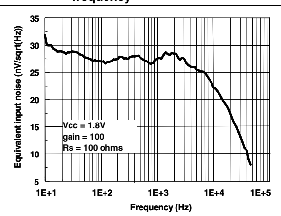
Figure 36. Equivalent input noise vs. frequency
