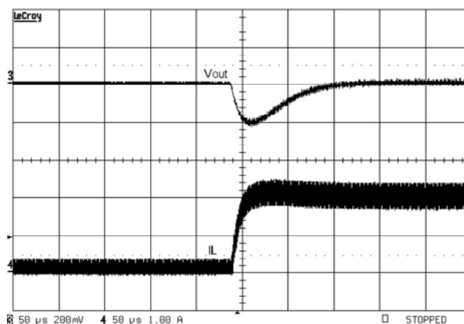
Figure 22. 100mA to 2A Load Step (Load Slew Rate=2.5A/ \mu s, V_{CC} =12V, V_{OUT} =4V)
