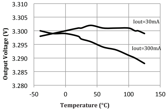
Figure 16. Output Voltage vs. Temperature
