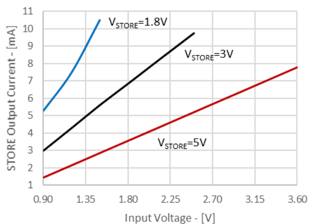
Maximum STORE Output Current vs Input Voltage w/ V_{STORE} \geq 96\% of Target: Circuit B
