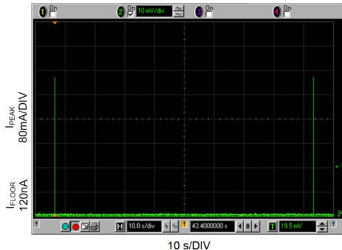
Input Quiescent Current : Circuit A with No-Load V_{IN}=3V , STORE=3V
