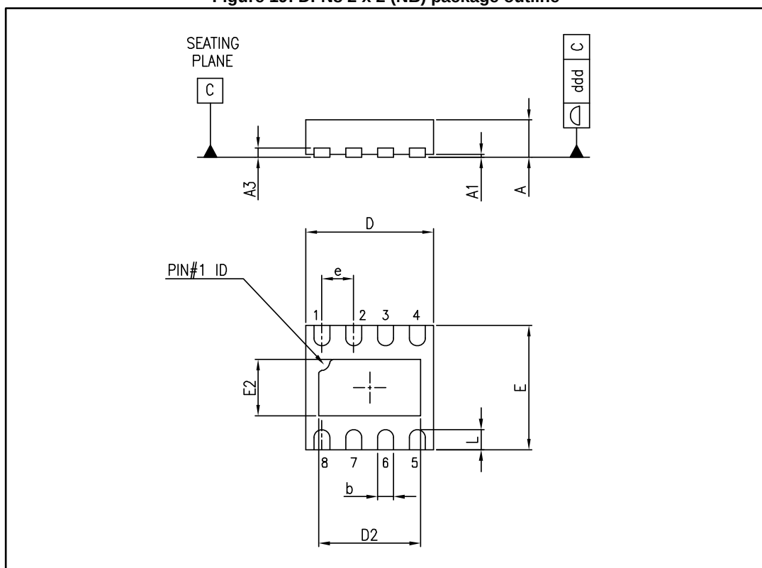
Figure 19: DFN8 2 x 2 (NB) package outline
