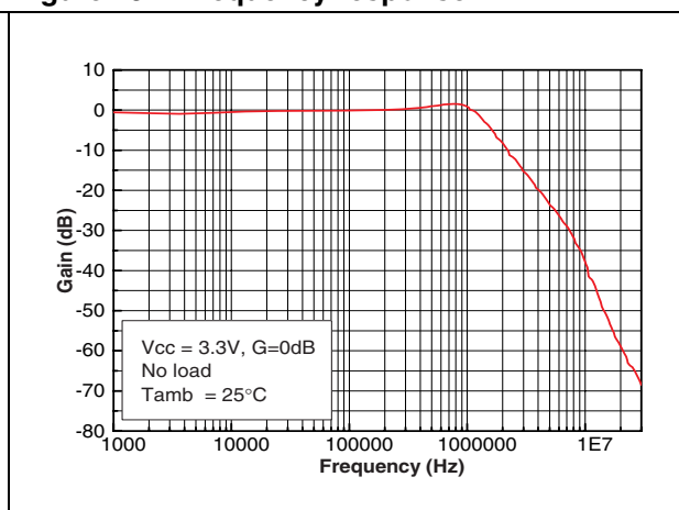
Figure 13. Frequency response
