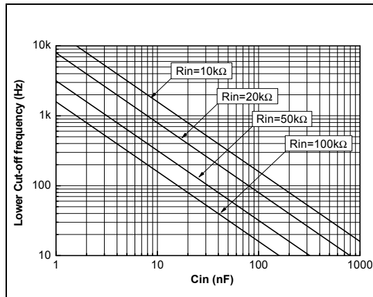
Figure 79. Lower cutoff frequency vs. input capacitor
