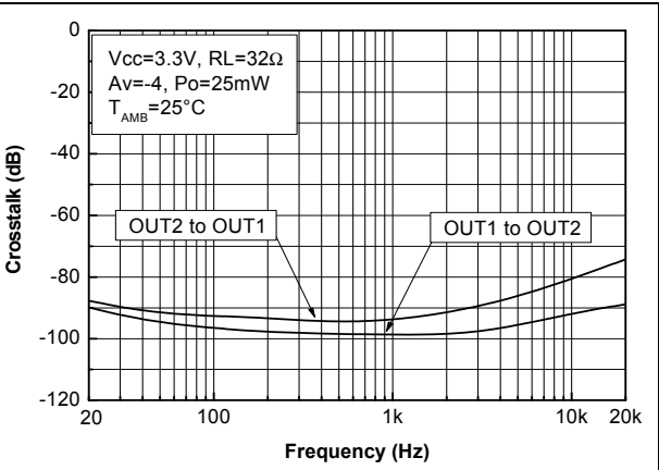
Figure 75. Crosstalk vs. frequency
