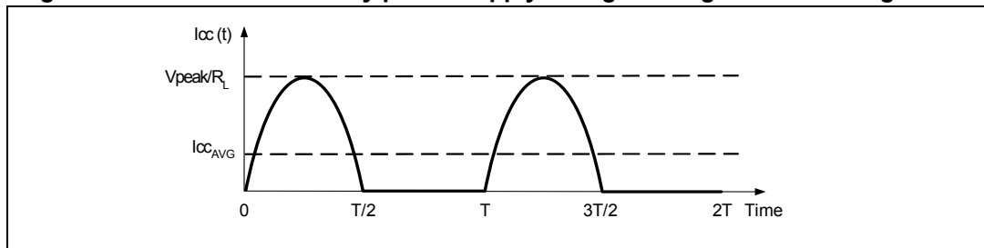
Figure 78. Current delivered by power supply voltage in single-ended configuration
