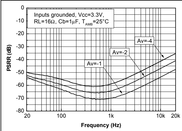
Figure 24. Power supply rejection ratio vs. frequency
