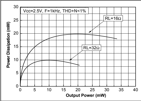
Figure 22. Power dissipation vs. output power per channel
