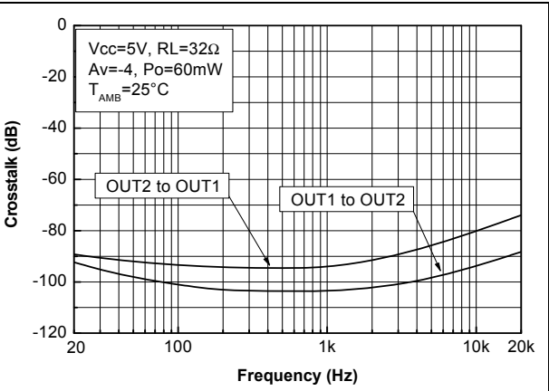
Figure 77. Crosstalk vs. frequency
