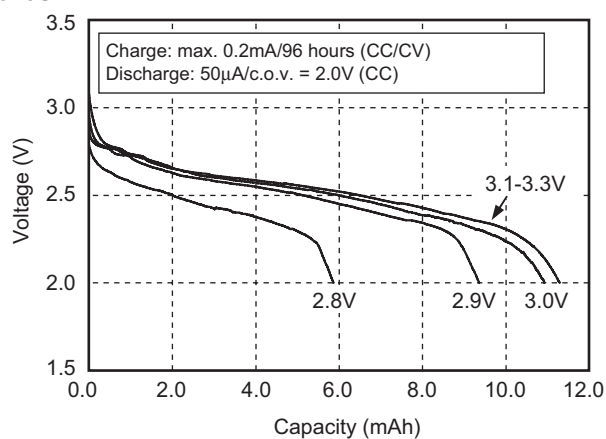
MS920SE
