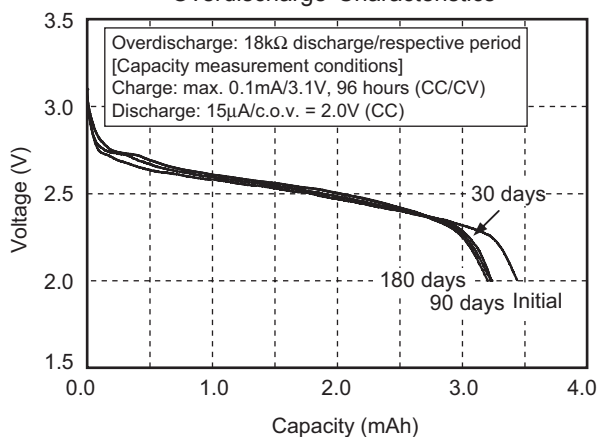
Overdischarge Characteristics
