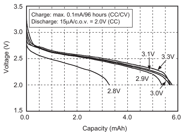
MS621FE
