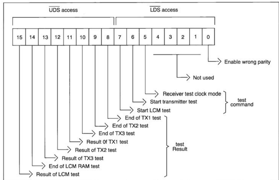
Figure 27. Self-test Register
