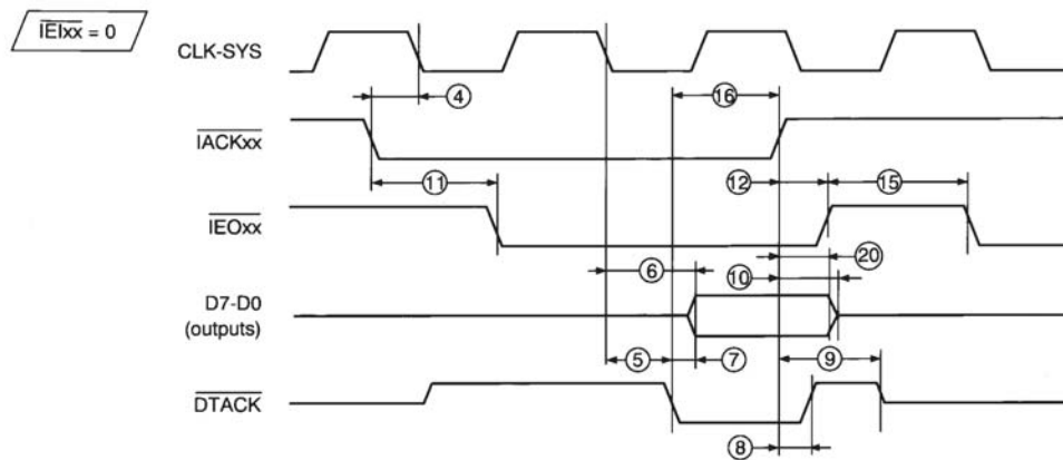
Figure 6. Interrupt Cycle ( \text{IEIxx} = 0 )
