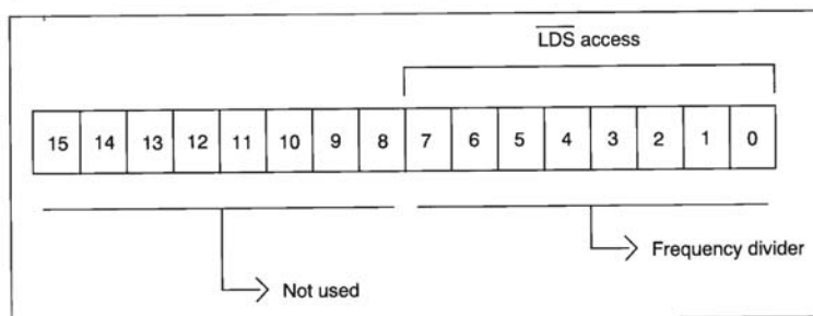
Figure 17. Frequency Register
