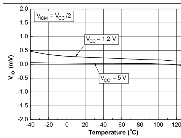
Figure 13. Input offset voltage vs. temperature Figure 14. Input hysteresis voltage vs. temperature
