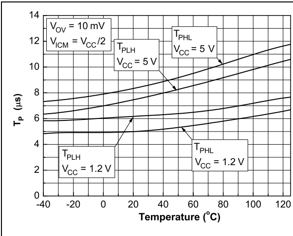
Figure 33. Propagation delay vs. temperature for signal overdrive 10 mV
