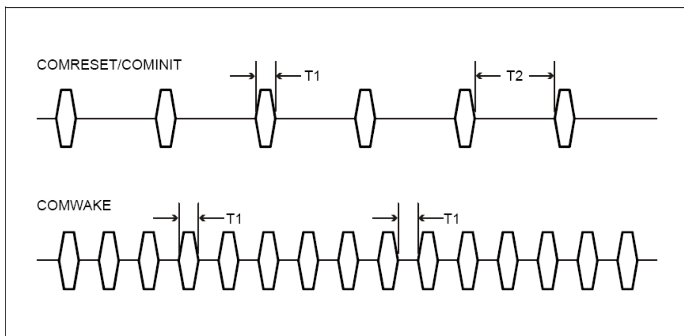
Figure 4 : OOB signals
