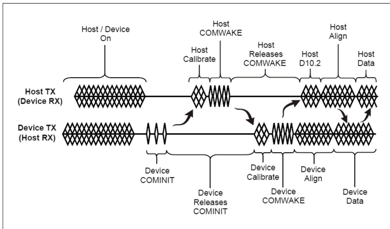
Figure 6 : cominit sequence
