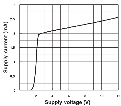
Figure 4. Total supply current vs. supply voltage
