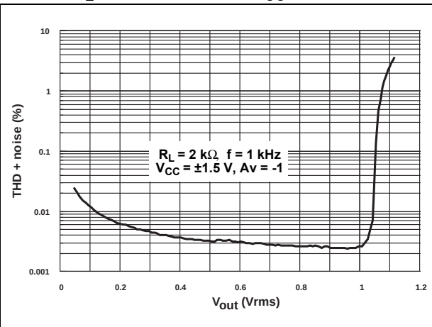
Figure 12. THD + noise vs. output voltage ( R_L = 2\text{ k}\Omega , f = 1\text{ kHz} , V_{CC} = \pm 1.5\text{ V} )
