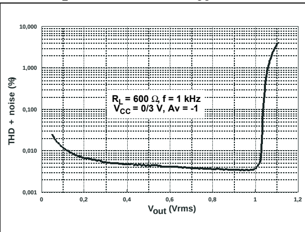
Figure 10. THD + noise vs. output voltage ( R_L = 600\ \Omega , f = 1\text{ kHz} , V_{CC} = 0/3\text{ V} )
