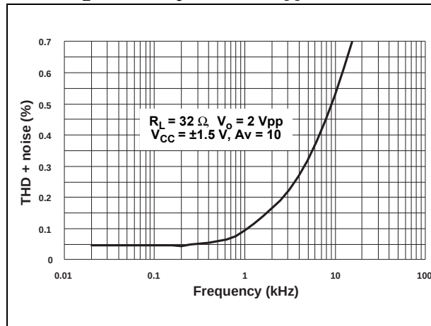
Figure 9. THD + noise vs. frequency ( R_L = 32\ \Omega , V_o = 2\text{ Vpp} , V_{CC} = \pm 1.5\text{ V} )
