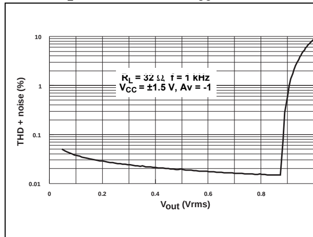
Figure 11. THD + noise vs. output voltage ( R_L = 32\ \Omega , f = 1\text{ kHz} , V_{CC} = \pm 1.5\text{ V} )
