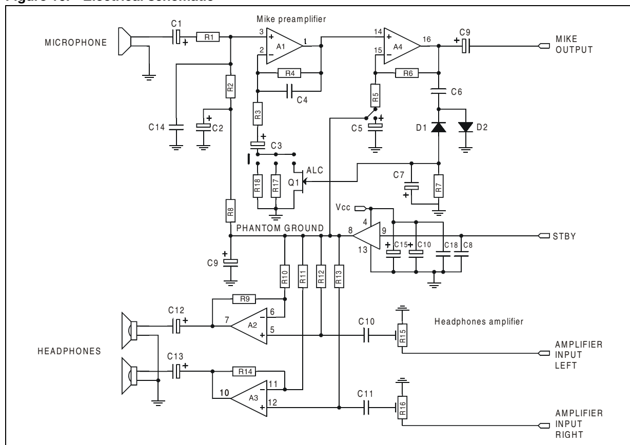
Figure 16. Electrical schematic
