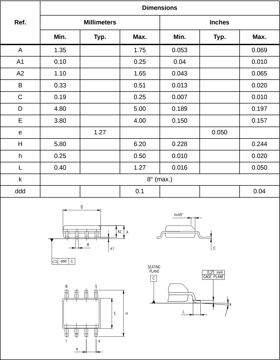
Figure 24. SO-8 package
