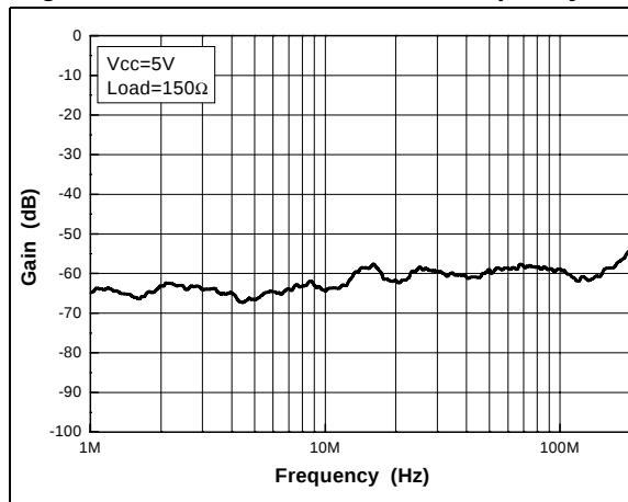
Figure 13. Reverse isolation vs. frequency
