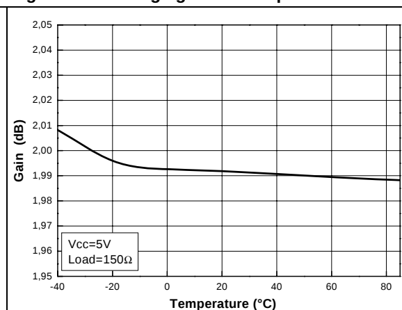
Figure 18. Voltage gain vs. temperature
