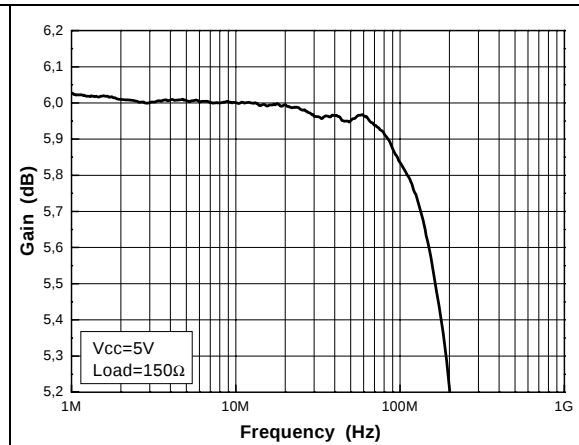
Figure 2. Gain flatness
