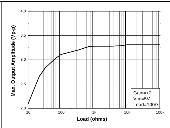
Figure 8. Output amplitude vs. load
