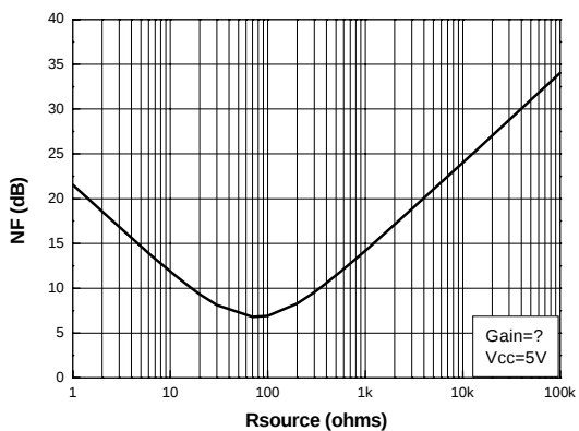
Figure 16. Noise figure
