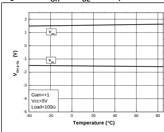
Figure 27. V_{OH} and V_{OL} vs. temperature
