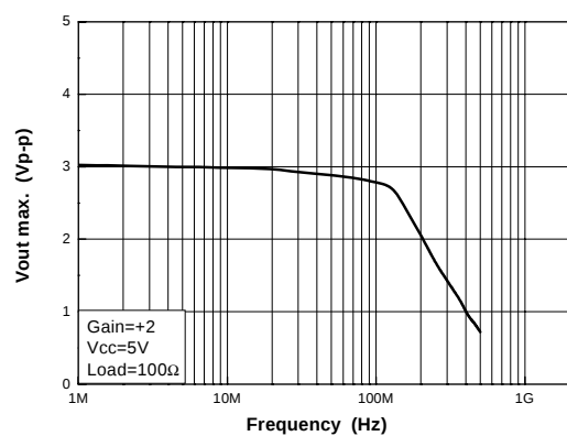
Figure 18. Output amplitude vs. frequency
