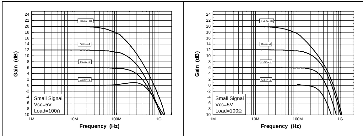
Figure 1. Frequency response, positive gain Figure 2. Frequency response, negative gain
