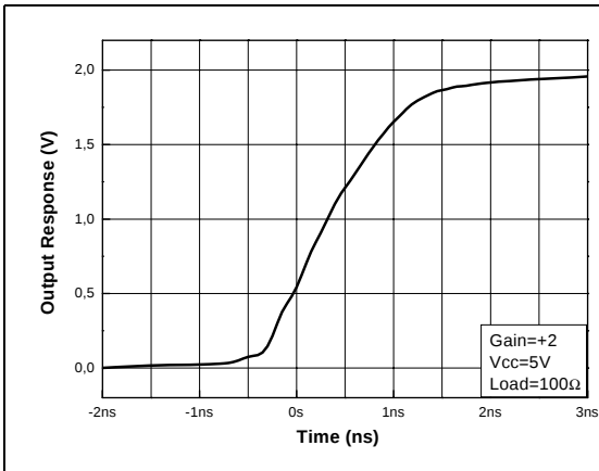
Figure 7. Slew rate
