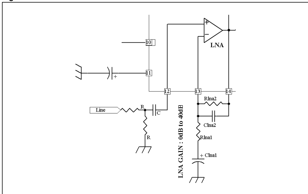
Figure 26. LNA schematics
