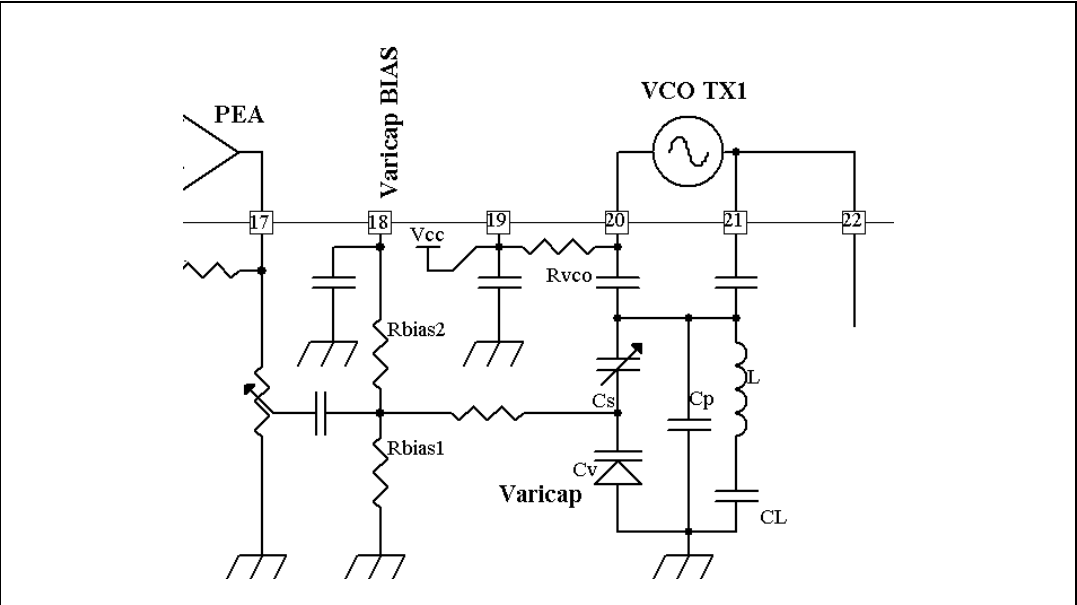
Figure 33. VCO schematics
