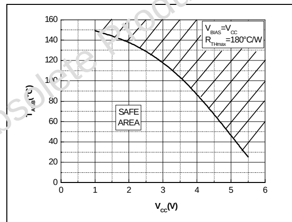
Figure 2 : Maximum T_{amb} vs V_{CC}
