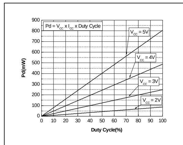
Figure 3 : Dissipation vs Duty cycle
