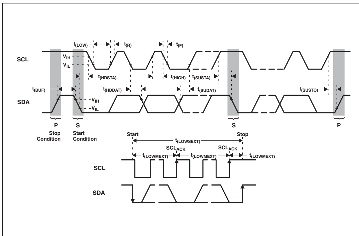
Figure 11: Timing Diagrams
