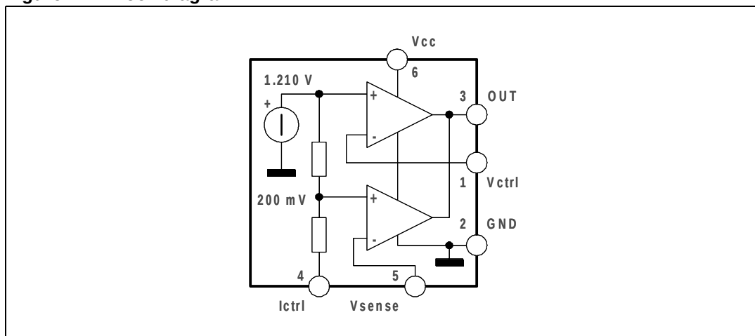
Figure 2. Block diagram
