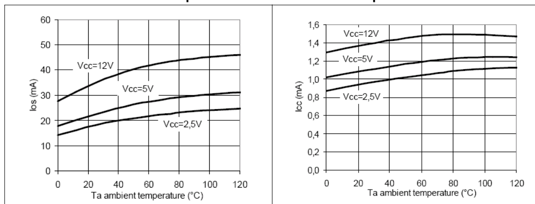
Figure 8. Output short circuit current Vs. Ambient Temperature Figure 9. Supply current Vs. Ambient Temperature
