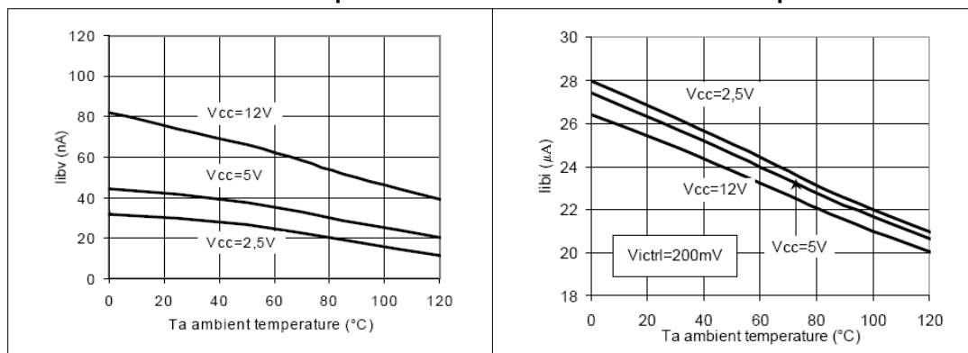
Figure 6. Vsense pin input bias current Vs. Ambient Temperature Figure 7. Ictrl pin input bias current Vs. Ambient Temperature
