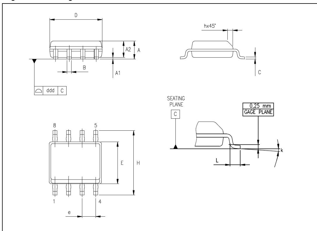
Figure 13. Package dimensions
