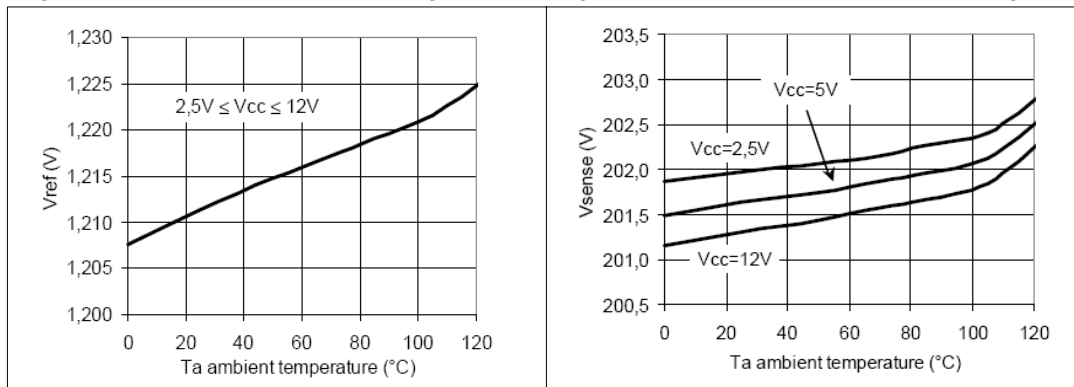
Figure 4. Vref Vs. Ambient Temperature Figure 5. Vsense Vs. Ambient Temp.
