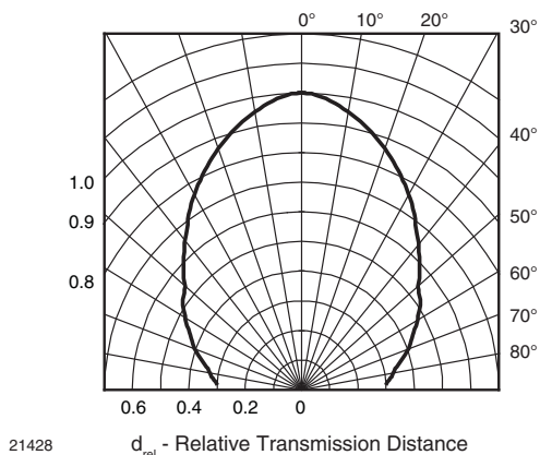
Fig. 4 - Vertical Directivity
