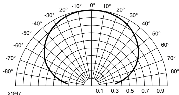
Fig. 11 - Directivity
