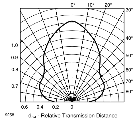
Fig. 12 - Horizontal Directivity
