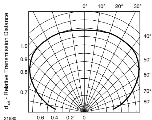
Fig. 12 - Vertical Directivity
