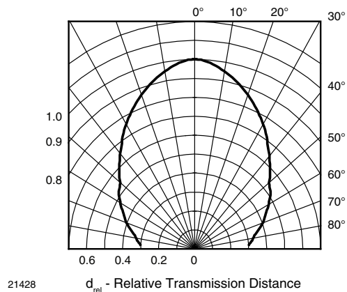
Fig. 12 - Vertical Directivity
