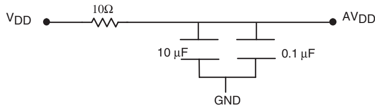
Figure 14-1. PLL Power Supply Filter Circuit
