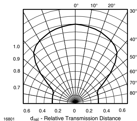
Fig. 8 - Horizontal Directivity
