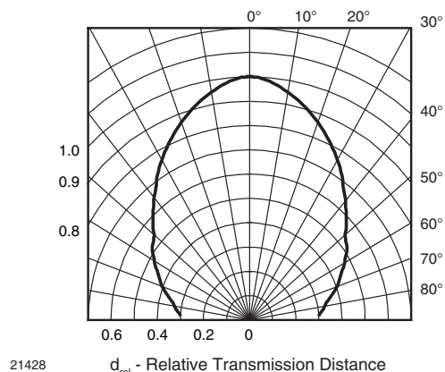
Fig. 9 - Vertical Directivity
