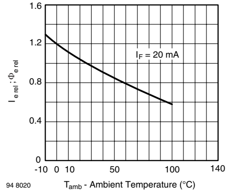
Figure 8. Rel. Radiant Intensity/Power vs. Ambient Temperature
