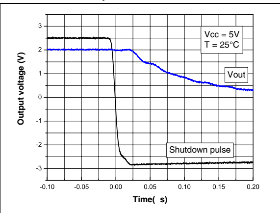
Figure 21. Turn-off time, V_{\text{CC}} = 5\text{ V} , Vout pulled down, T = 25^\circ\text{ C}
