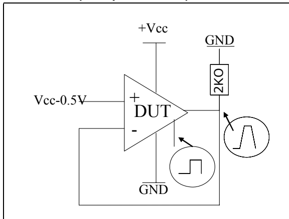
Figure 20. Turn-on time, V_{\text{CC}} = 5\text{ V} , Vout pulled down, T = 25^\circ\text{ C}
