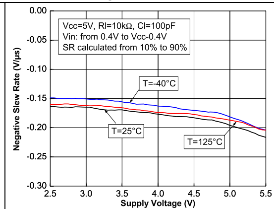
Figure 11. Negative slew rate vs. supply voltage
