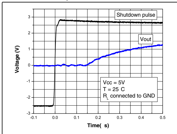
Figure 20. Turn-on time, V_{\text{CC}} = 5\text{ V} , Vout pulled down, T = 25^\circ\text{ C}
