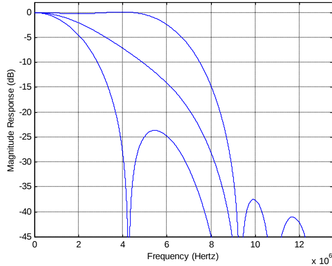
FIGURE 62 CHARACTERISTICS OF LUMINANCE FILTER
