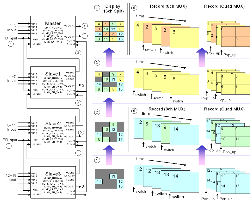
FIGURE 49 THE CASCADE CONNECTION FOR 240 CIF/SEC RECORD MODE
