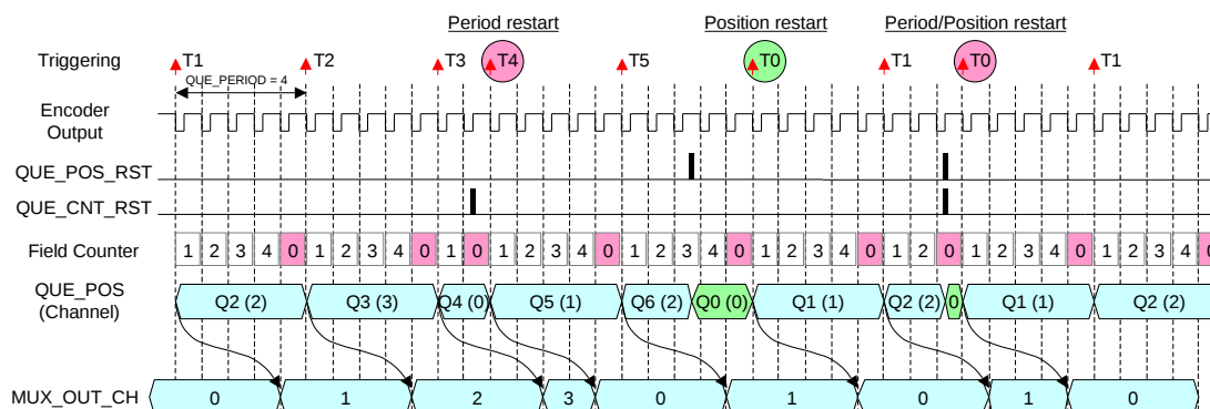
FIGURE 24 THE ILLUSTRATION OF QUE POS RST AND QUE CNT RST
