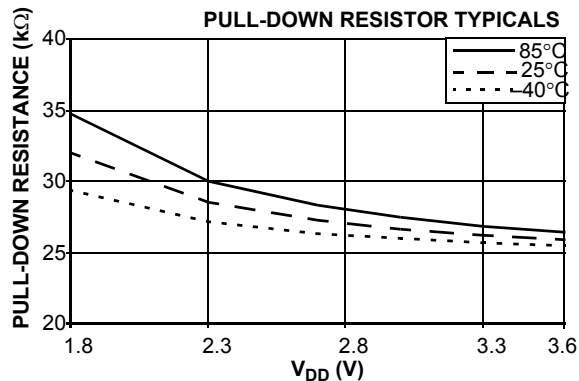
Figure 5. Pull-up and Pull-down Typical Resistor Values
