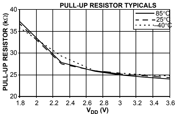
Figure 5. Pull-up and Pull-down Typical Resistor Values
