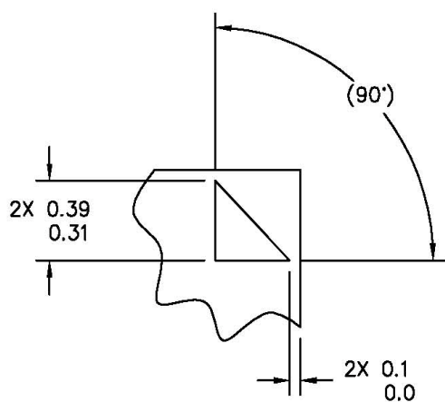
DETAIL T
