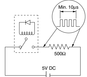
Measuring condition of M.B.B. time
