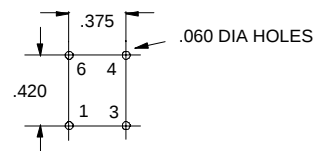
UNIT MOUNTING PATTERN
