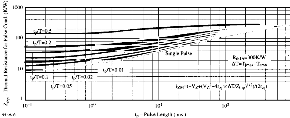
Figure 10 : Thermal Response
