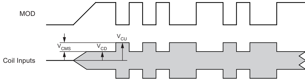
Figure 4-1. Modulation
