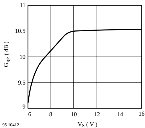
Figure 7. G_{RF} vs. V_S
