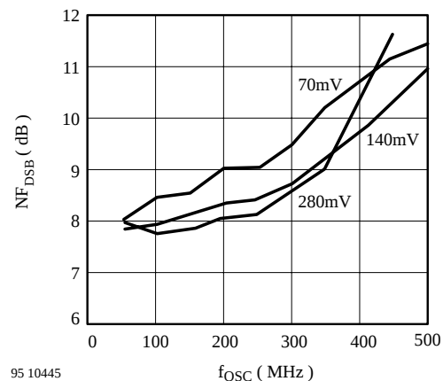
Figure 49. NF_{DSB} vs. f_{OSC}
