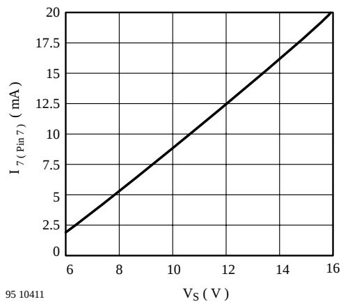
Figure 6. I_7 vs. V_S
