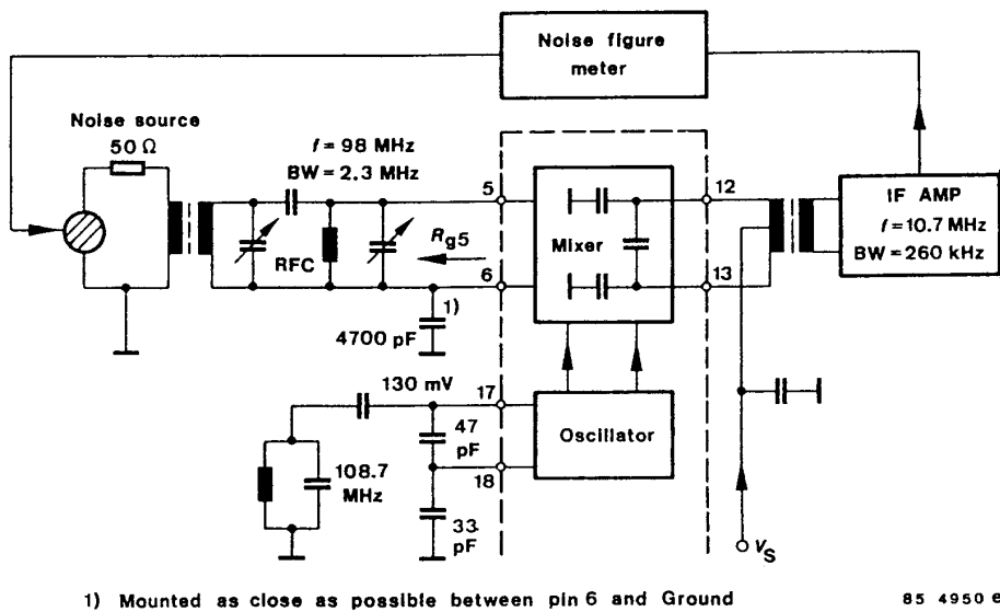
Figure 26. Test circuit for single sideband noise ( F_{CSSB} )
