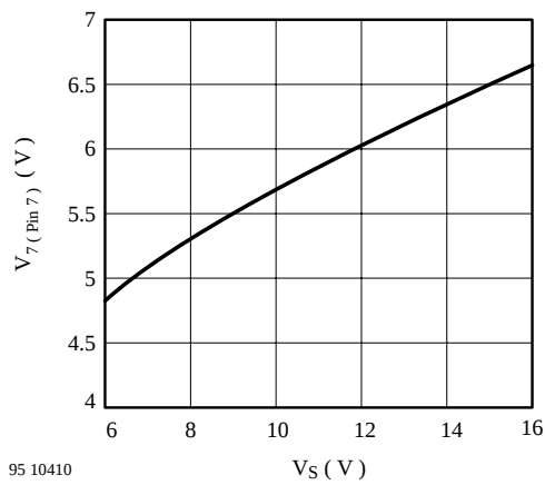
Figure 5. V_7 vs. V_S
