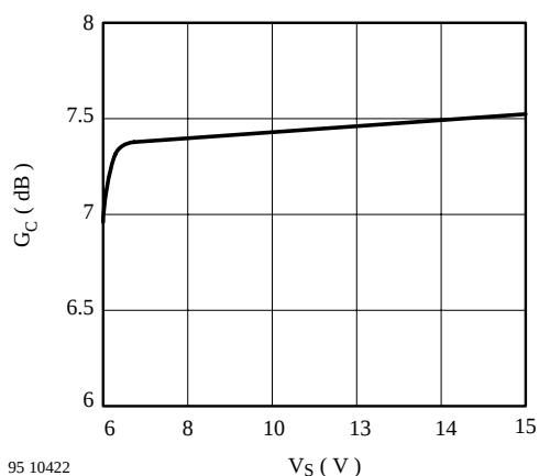
Figure 19. G_C vs. V_S
