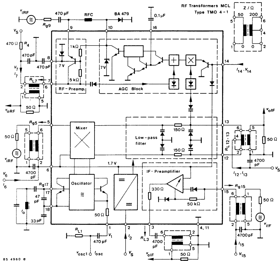
Figure 3. Test circuit
