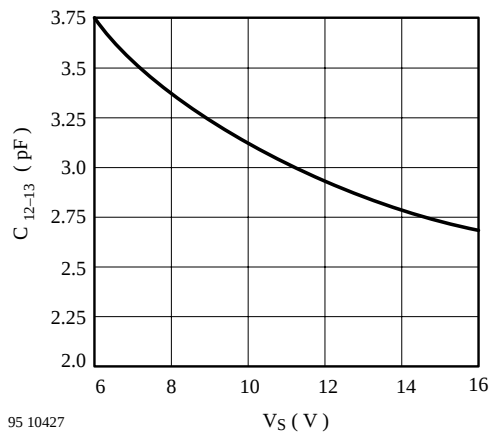
Figure 24. C_{12-13} vs. V_S
