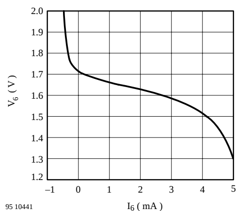
Figure 42. V_6 vs. I_6
