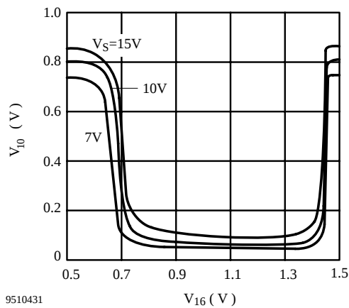
Figure 30. V_{10} vs. V_{16}
