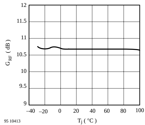
Figure 8. G_{RF} vs. T_j
