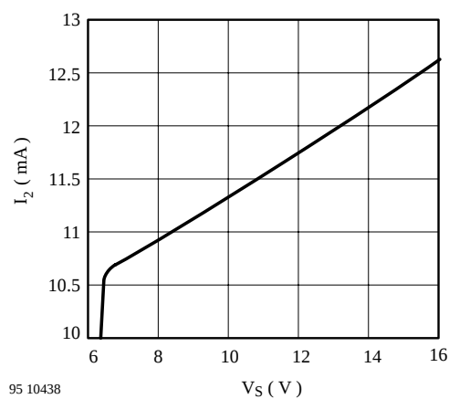
Figure 39. I_2 vs. V_S
