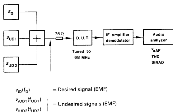
Figure 44. Block diagram of the test set up
