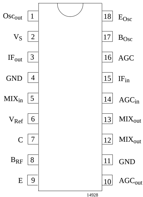
Figure 2. Pinning DIP18
