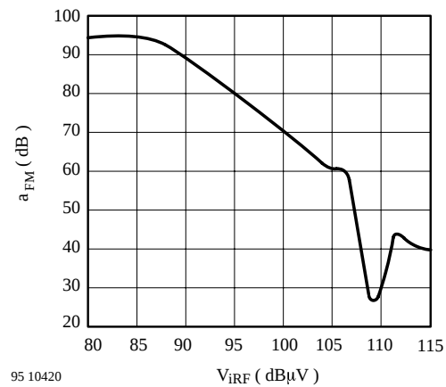
Figure 16. a_{\text{FM}} vs. V_{i\text{ RF}}
