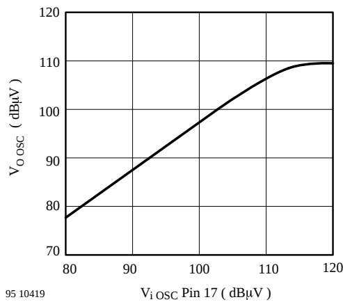
Figure 15. V_{O\text{ OSC}} vs. V_{i\text{ OSC}}
