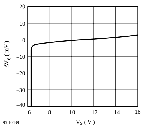
Figure 40. \Delta V_6 vs. V_S
