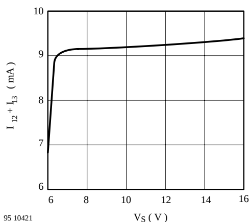
Figure 18. I_{12} + I_{13} vs. V_S
