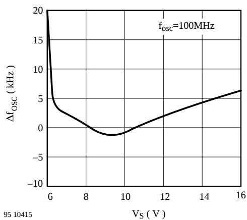
Figure 11. \Delta f_{osc} vs. V_S
