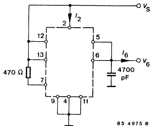
Figure 38. Test circuit
