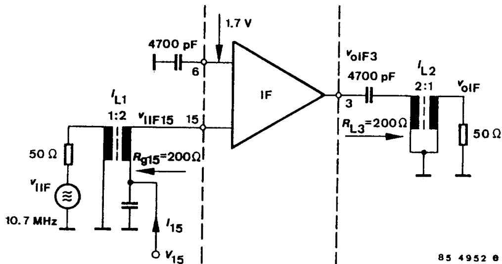
Figure 32. Test circuit
