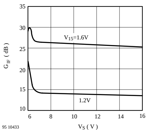
Figure 33. G_{IF} vs. V_S
