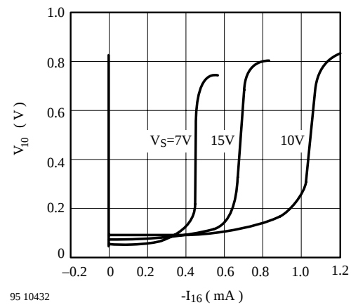
Figure 31. V_{10} vs. -I_{16}
