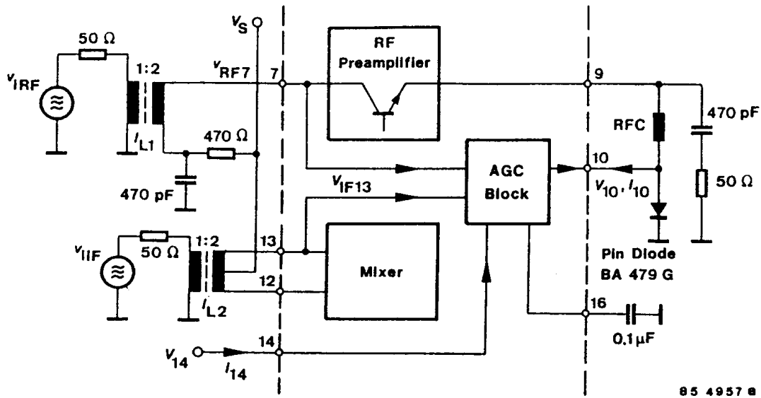
Figure 27. Test circuit
