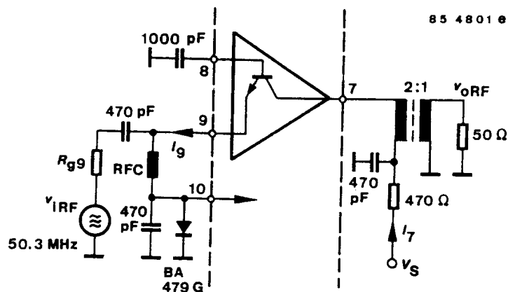
Figure 4. Test circuit
