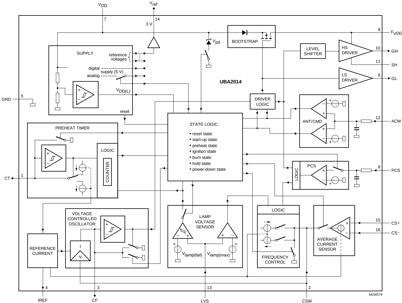
Fig.1 Block diagram.
