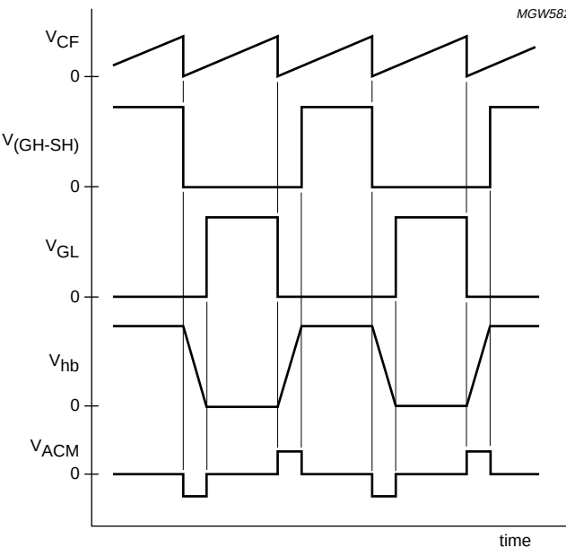
Fig.4 Oscillator and driver signals.
