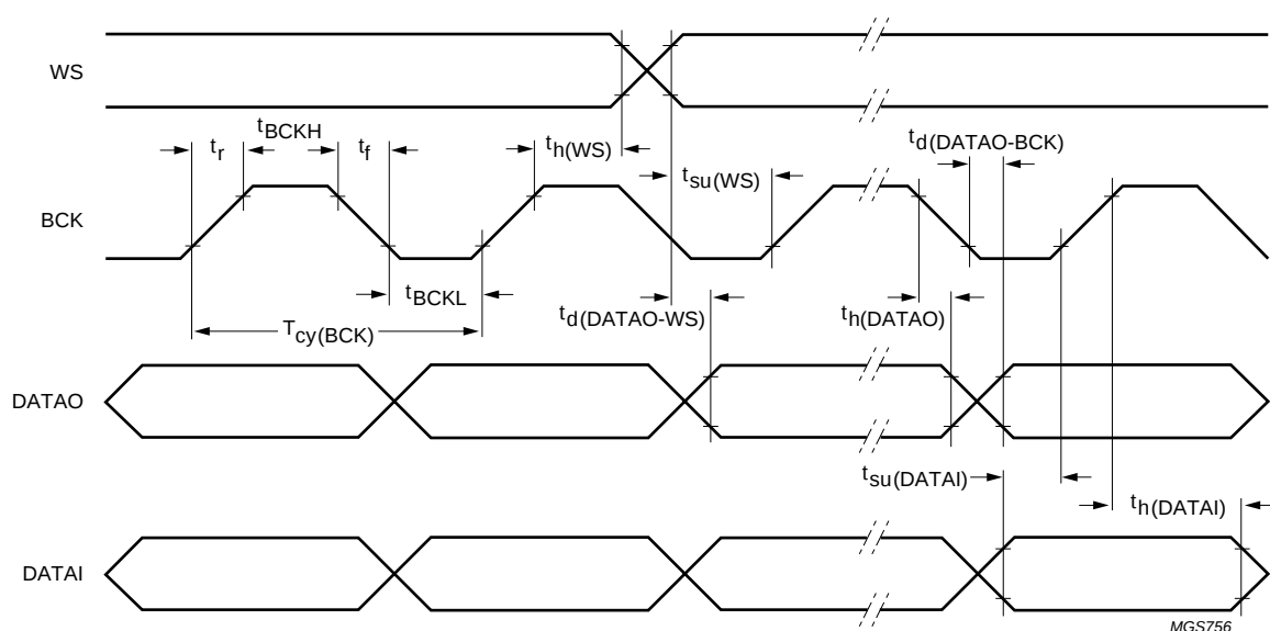
Fig.8 Serial interface timing.
