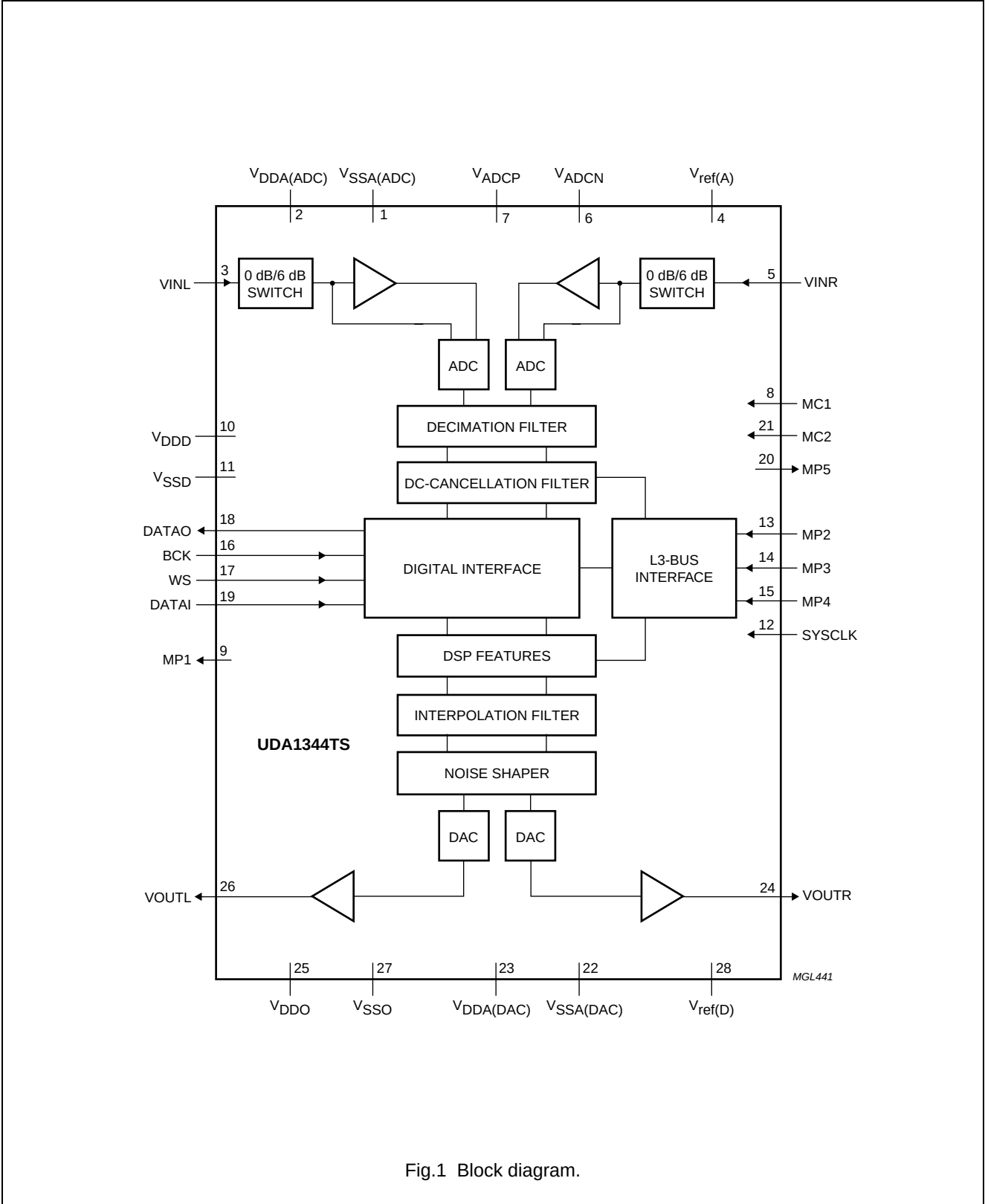
BLOCK DIAGRAM
