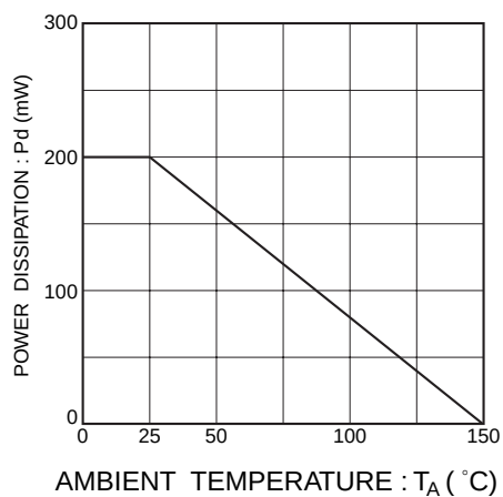
Fig.2 Derating curve
