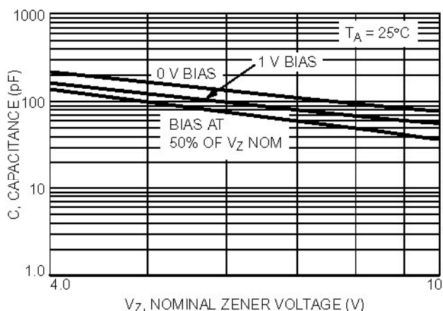
Figure 3. Typical Capacitance
